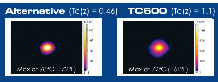
Figure 3 - THERMAL COMPARISON – thermal image of 25 mil laminate test circuit
